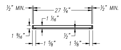
SECTION THROUGH ANGLE FRAME FOR STANDARD No. 2-2-A CATCH BASIN
