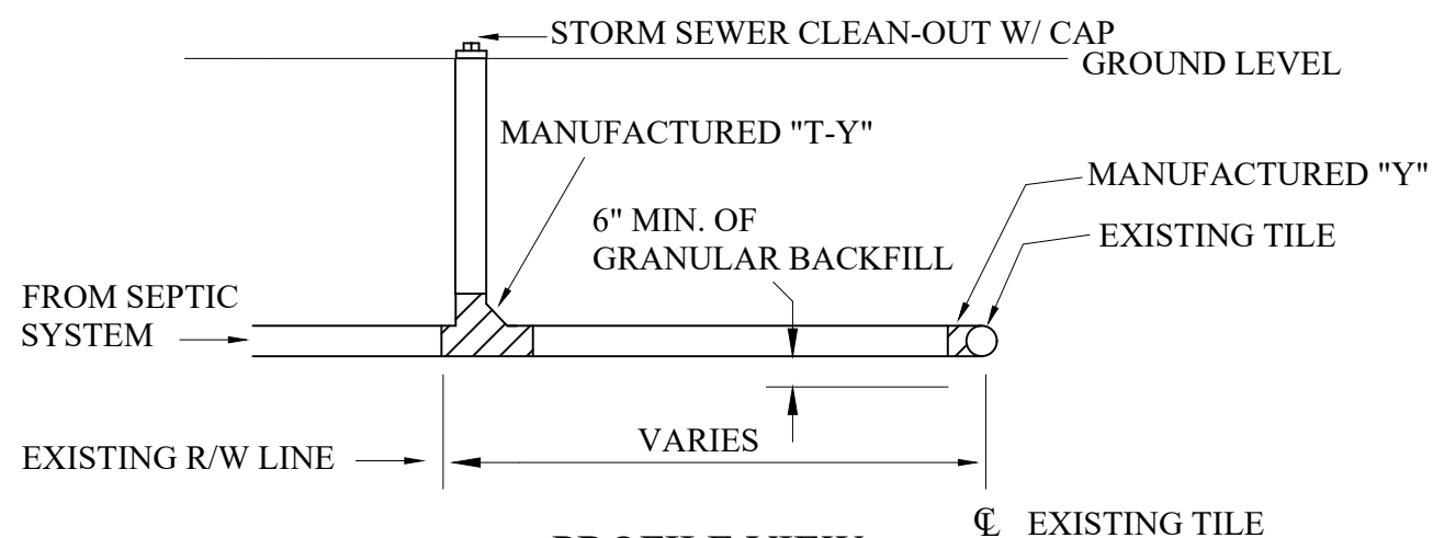
PROFILE VIEW
