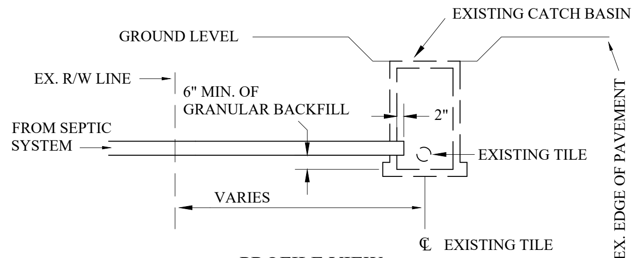
PROFILE VIEW
